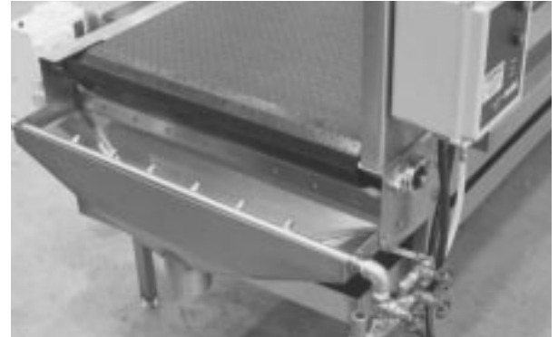
Spray bar at discharge of machine cleans shrimp off belt. Water conveys shrimp to the next machine in the line.
